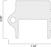
Frosted channel endcap - wired end
