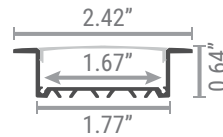
Height with Lens 0.69"
